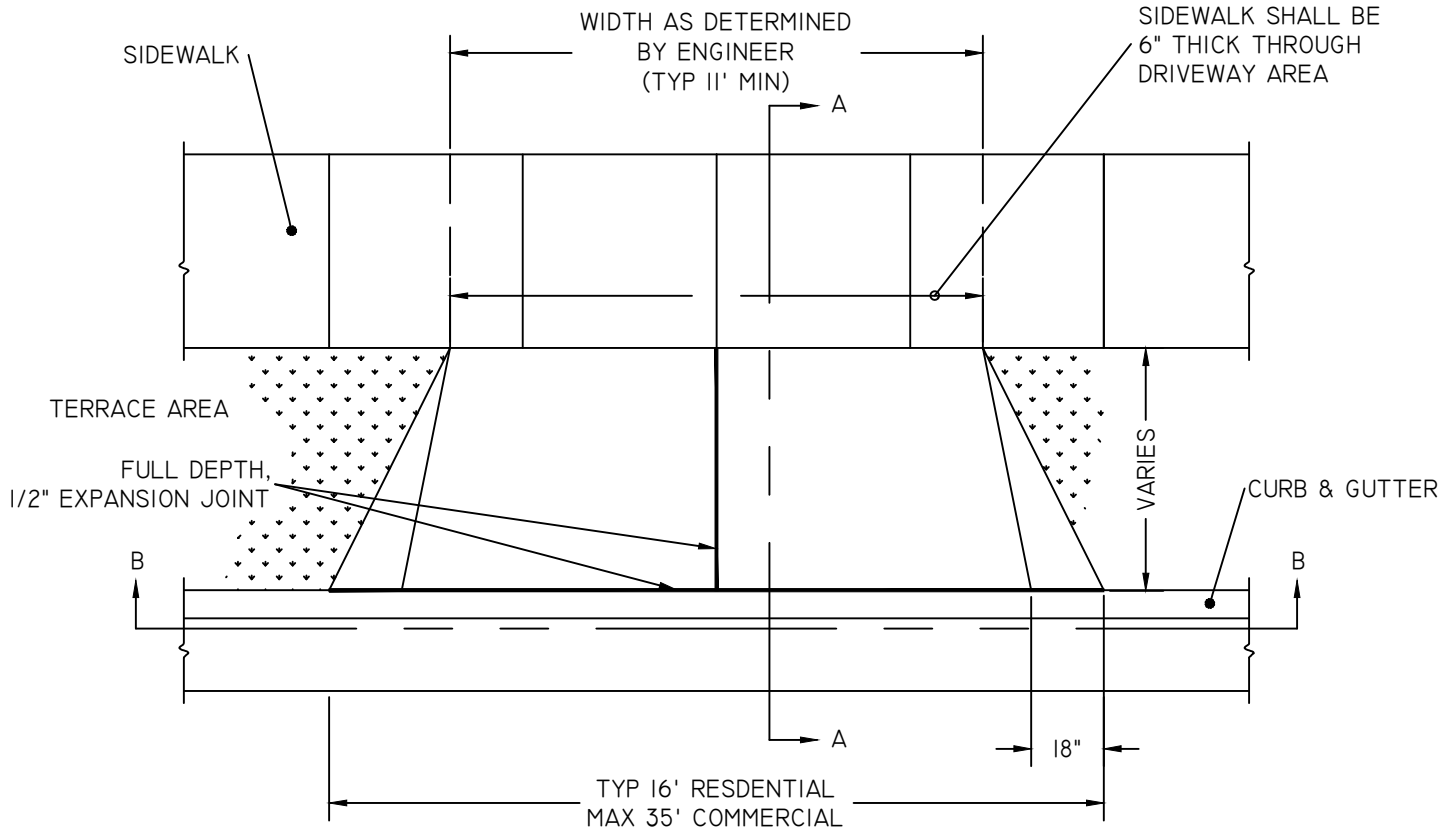
DRIVEWAY PLAN
