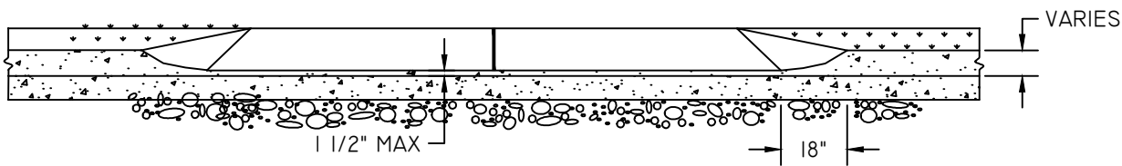
SECTION B-B
