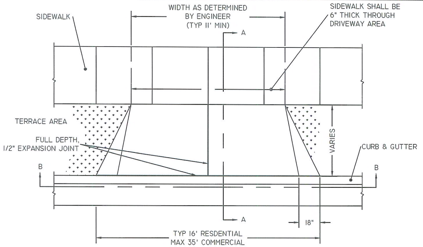
DRIVEWAY PLAN
